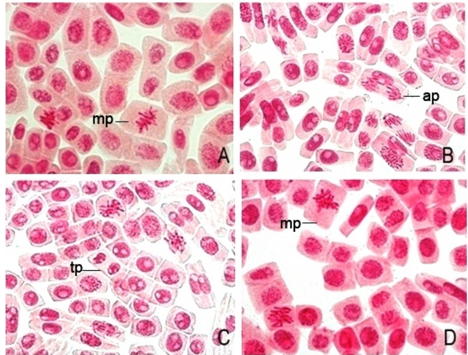
Figure 1: Mitotic cell division of Allium cepa root tip cells at 24 hrs, (A), Control; (B-D), test solutions. pp , prophase; mp , metaphase; ap , anaphase; tp , telophase.
