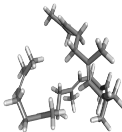
Figure 2: 3D structure of Squalene
