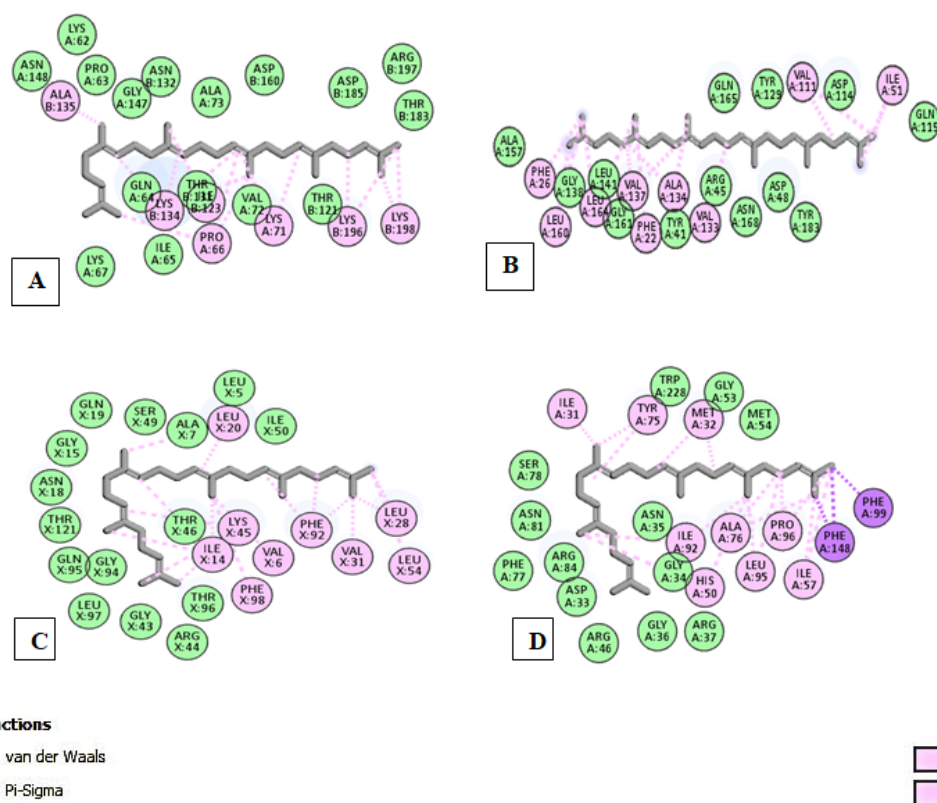
Figure 6: 2D representation of interaction between Squalene and target proteins A (1T2P), B (2ZCO), C (3FYV) and D (4H8E)
