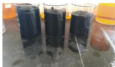
Figure 3.3: Adsorption Trials.
