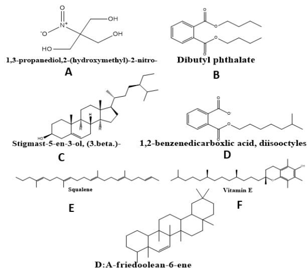
Figure 4: Structure of some valuable novel bioactive compounds from calli of Argemone mexicana stem (NIST and PUBCHEM); 4A: 1,3 propanediol,2-(hydroxymethyl)-2-nitro-; 4B: Dibutyl phthalate; 4C: Stigmast-5-en-3ol, (3- beta); 4D: 1,2-benzenedicarboxylic acid, diisooctyles; 4E: Squalene; 4F: Vitamin E; 4G: D: A-friedoolean-6-ene
