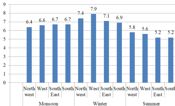
Fig 2: Flucuating Levels of Dissolved Oxygne (mg/L)
