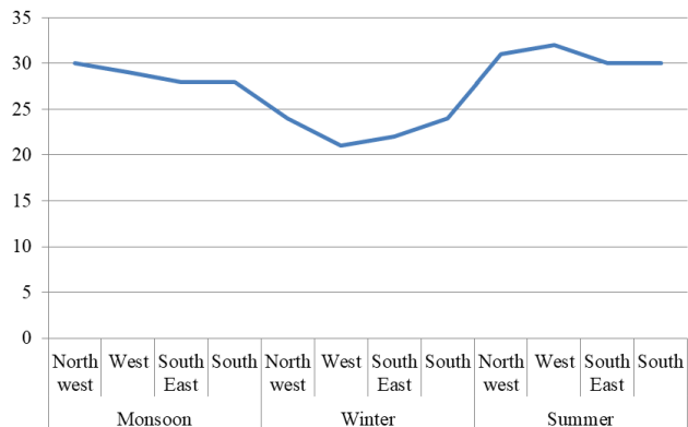
Fig 1: Temperature of lake waters during different seasons (in °C)
